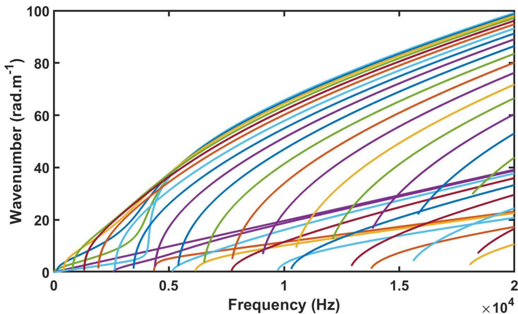
Figure 7: Dispersion curves of the pipe
