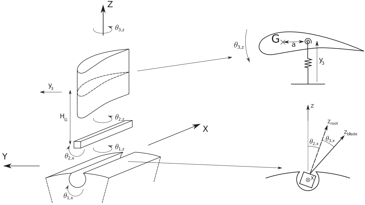
Figure 7: Phenomenological model of a bending-torsion blade with dry friction at blade root
