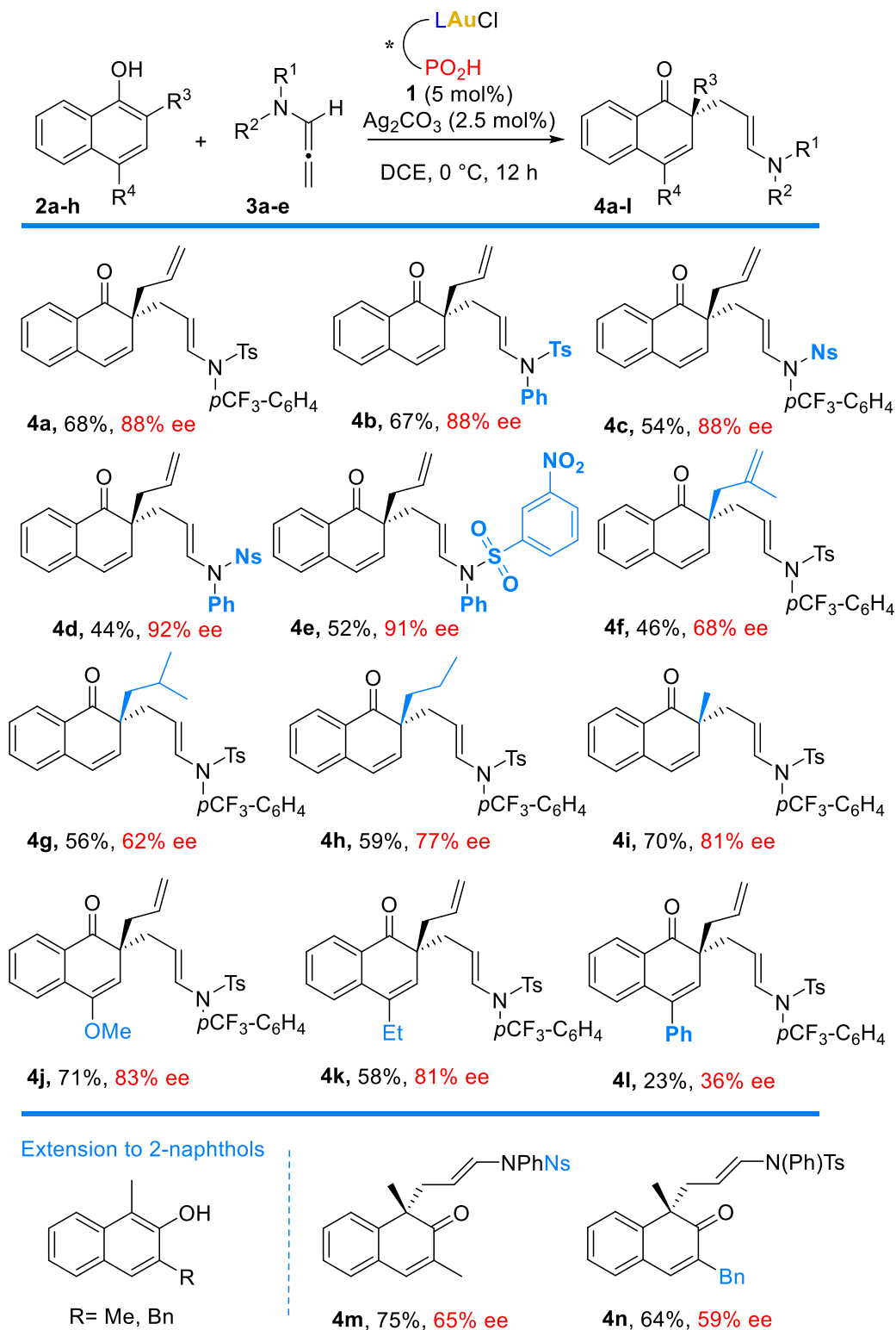
Scheme 2: Scope of the enantioselective dearomatization of 1- and 2-naphthols with allenamides, using pre-catalyst (CPAPhos A )AuCl, 1 .
