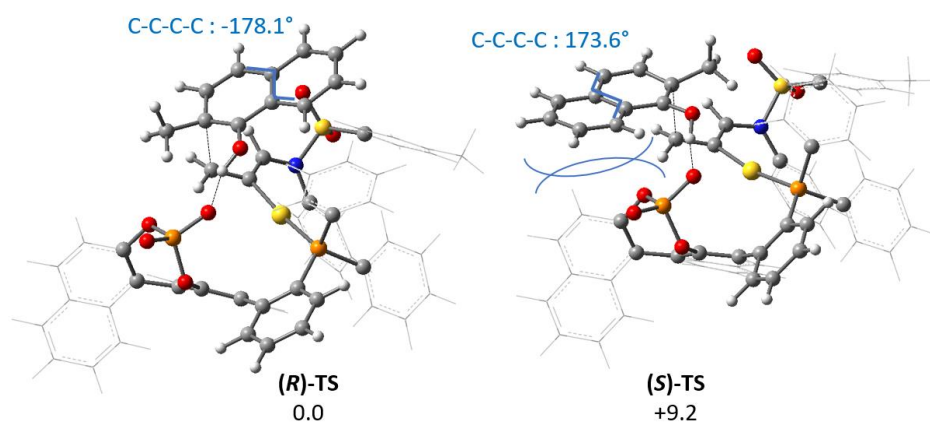
Figure 2: Optimized geometry of transition states connecting intermediate 8 and 9 . Relative Gibbs free energy (in kJ/mol). For clarity, a wire frame representation of some aryl groups is used.
