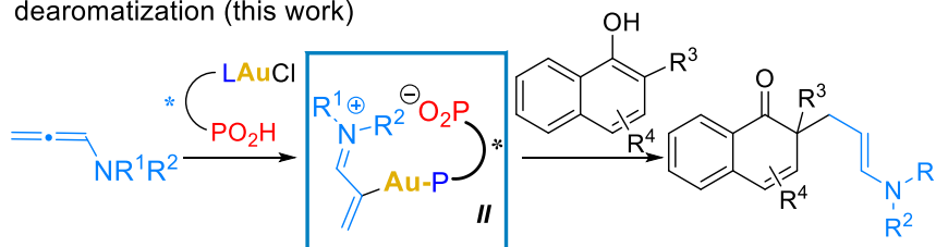
Scheme 1: Models for the stereochemical control in reactions involving pre-catalyst 1
