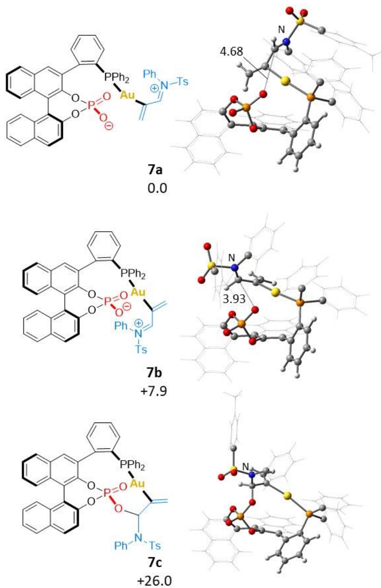
Figure 1: Selected optimized geometries of intermediates 7 . Relative Gibbs free energy (in kJ/mol).
