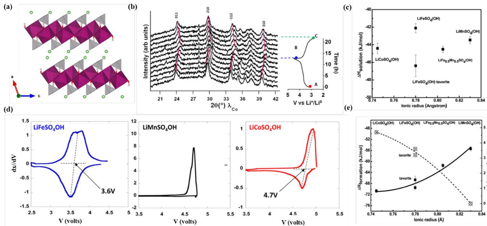
Figure 5. Structure and electrochemical properties of layered hydroxysulfates \text{LiMSO}_4\text{OH} ( \text{M}=\text{Fe} , \text{Mn} , \text{Co} ). (a) Structure built with \text{MO}_6 octahedra (maroon) and \text{SO}_4 tetrahedra (grey) delimiting voids for Li atoms (green sphere). (b) In-situ XRD patterns of layered \text{LiFeSO}_4\text{OH} . (c) enthalpy of dissolution of \text{LiMSO}_4\text{OH} compounds in 5 M HCl at 25 ^\circ C. (d) Derivative curves showing the respective redox potential. (e) enthalpies of formation (solid curve with square symbols) along with redox potentials (dashed lines with diamond symbols) as a function of cation radius. (b),(d) Reproduced with permission. 78 Copyright 2013, American Chemical Society (c), (e) Reproduced with permission. 82 Copyright 2014, The Royal Society of Chemistry.
