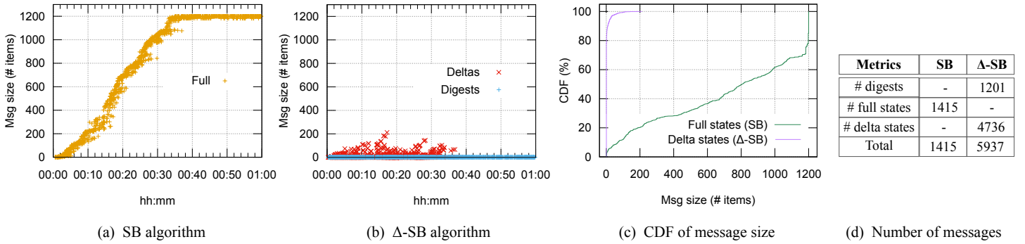
Figure 1: AW-Set synchronization
