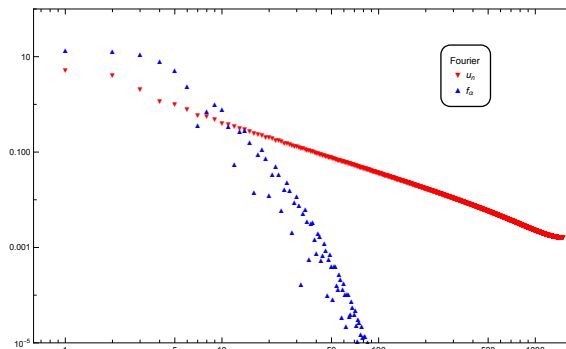
FIGURE 2. Typical frequency profile (modulus of the Fourier transform against the frequency) of a function u_n and f_\alpha from Figure 1. An FFT was performed on a discretized version of each function. The units are arbitrary and in log-log scale.
