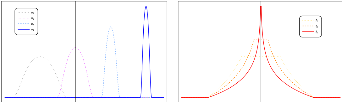
FIGURE 1. Left: a typical sequence (u_n) illustrating the default of compactness due to the simultaneous effect of translations (1.5) and concentration (1.6). Right: a few terms of Moser's (f_\alpha) sequence (1.8).
