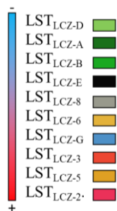
Figure 9. Distribution of LCZs of the study area from lowest to highest LST.
