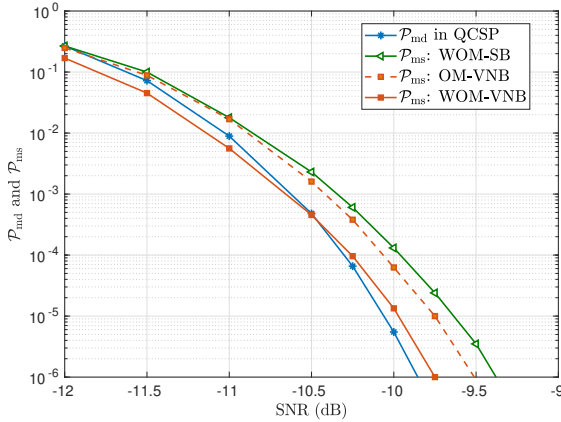
Fig. 6. \mathcal{P}_{\text{md}} and \mathcal{P}_{\text{ms}} vs SNR for the QCSP receiver using several combinations of the symbol and chip synchronization methods.
