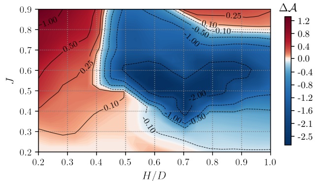
FIG. 3: Difference in wear damage \Delta\mathcal{A} between ductile ( r_y = 6 ) and quasi-brittle ( r_y = 0.5 ) junctions.
