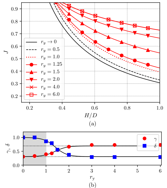
FIG. 5: (a) Criterion (2). (b) Coefficients \gamma and \delta : computed values (symbols) and predictions (3) with s = 1.4 , w = 0.25 and \mathcal{C} = 0.3 . Dotted lines in (b) mark the plateau values at \mathcal{C} and 1 - \mathcal{C} .
