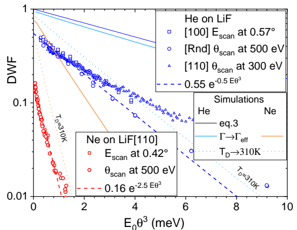
FIG. 6. The DWF, measured as the relative intensity of elastic diffraction, is reported for He and Ne projectiles on LiF along various orientations as a function of E\theta^3 . The ( \circ , \circ ) symbols were recorded on the same surface and the associated dashed lines are only to guide the eye outlining the effect of the projectile mass on the decay constant. The ( \Delta ) symbols correspond to a different target suggesting a possible influence of the surface coherence length (defect density). The simulations are described in the discussion.
