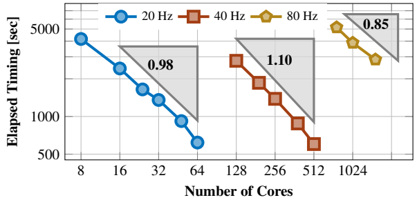
Figure 2: Point source at f = 20, 40 , and 80 Hz: total elapsed timing spent in the CMCG method by increasing the total number of cores.
