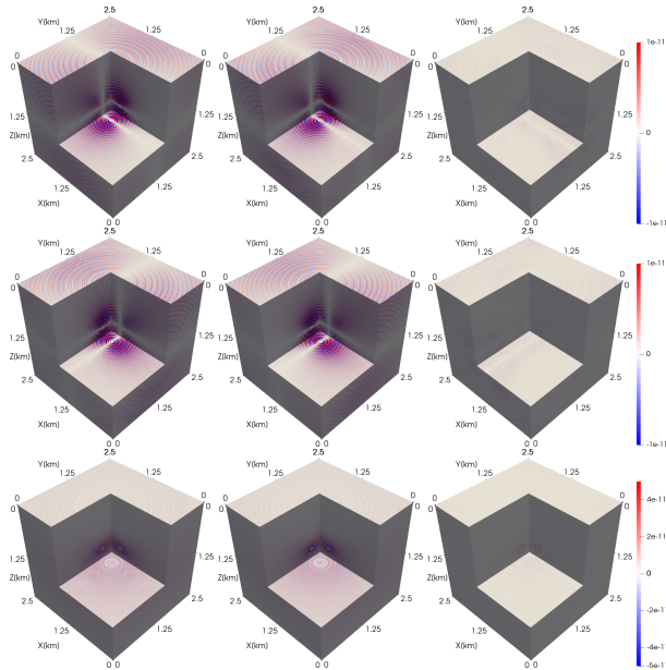
Figure 4: wavefields u_x (1st row), u_y (2nd row), and u_z (3rd row) of the point source problem of 80Hz, obtained with the CMCG method (1st column), the analytical solutions (2nd column), and the analytical errors (3rd column).
