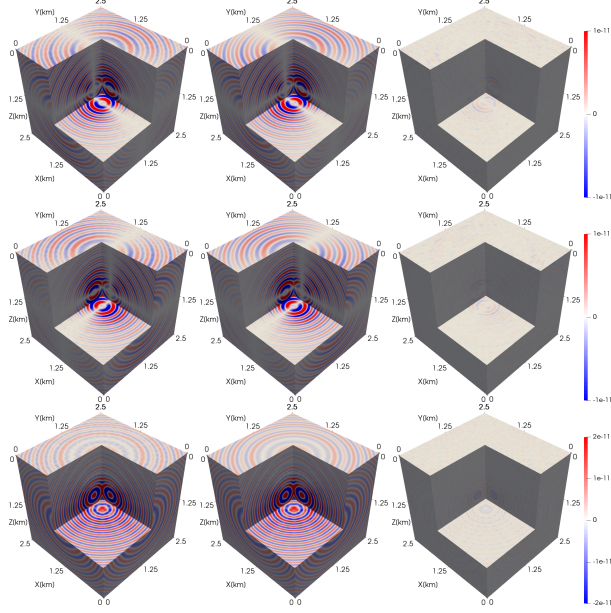
Figure 1: Wavefields u_x (1st row), u_y (2nd row), and u_z (3rd row) of the point source problem at 20[Hz], obtained with the CMCG method (1st column) and the direct solver (2nd column). The numerical differences between both methods are shown in the 3rd column.
