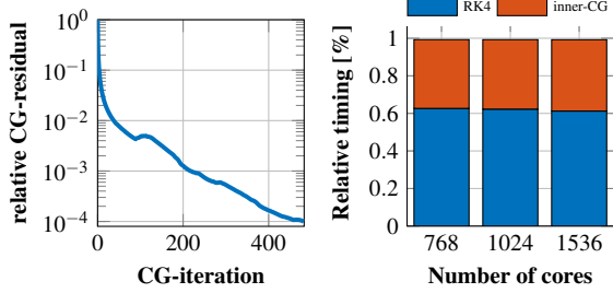
Figure 3: Pointsource 80Hz: (left) convergence of the outer CG loop; (right) elapsed timing in the inner CG loops and in the wave propagation solver (RK4).
