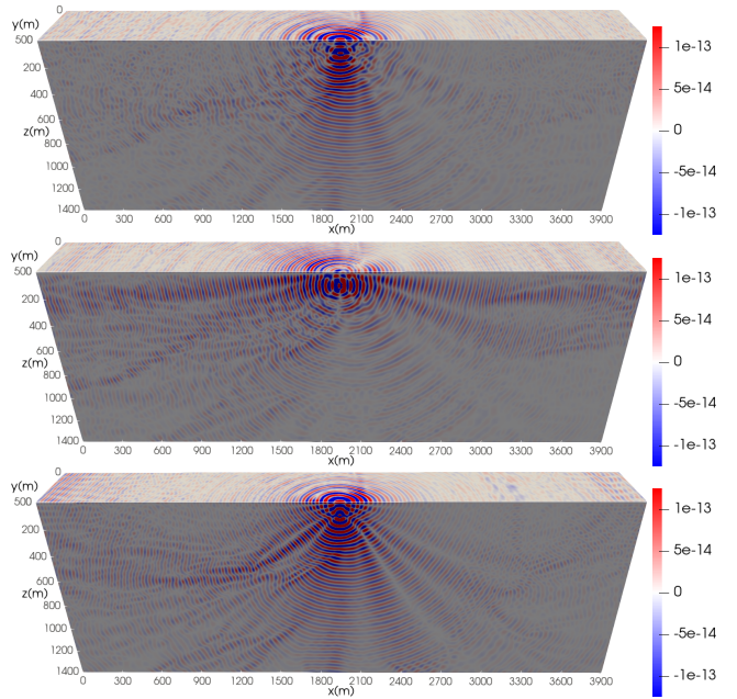
Figure 5: wavefields u_x (1st row), u_y (2nd row), and u_z (3rd row) of the Marmousi problem at 40Hz, obtained with the CMCG method.
