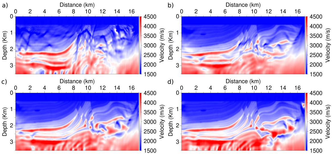
Figure 4: Final models after 400 iterations. L^2 inversion (a), l -BFGS GSOT inversion without preconditioning (b), l -BFGS GSOT inversion with pseudo-Hessian preconditioning (c), BFGS GSOT inversion with pseudo-Hessian preconditioning (d).
