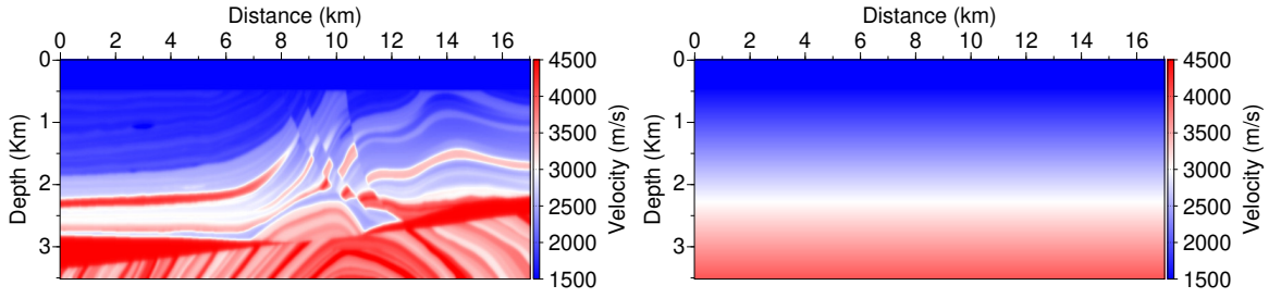
Figure 2: Exact (left) and initial (right) models.
