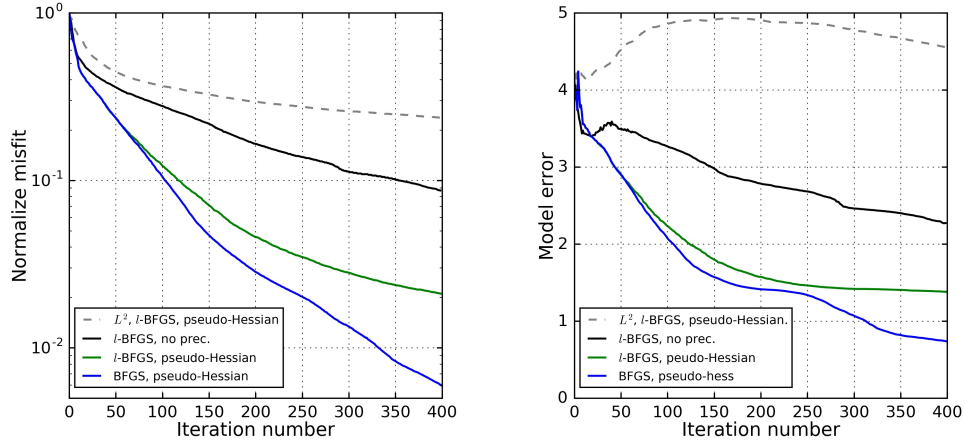
Figure 3: Convergence curves along FWI iterations. Normalized misfit functions (left), corresponding model error (right).
