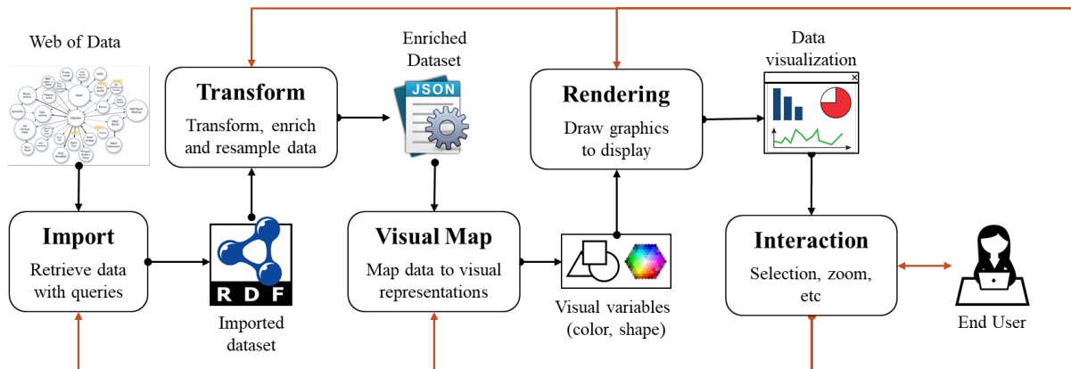
Figure 1: LOD generic visualization pipeline. Based on Telea (2014).
