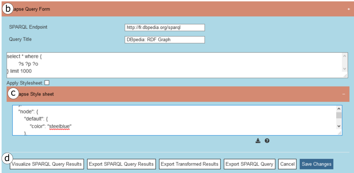
Figure 2: SPARQL Query Management Interface. (a) Listing of predefined queries. (b) The querying area. (c) The GSS editing area. (d) Control buttons to visualize and export the results.
