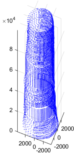
Figure 2: Example of a 3D full profile scan of a log
