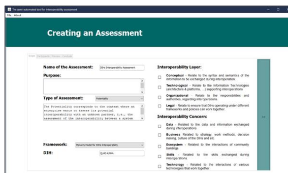
Figure 4: Screenshot of the DIHs assessment scope: Interoperability Barriers and Concerns
