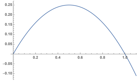
Figure 1: The plot of \tilde{\phi} . In this case we have \bar{\tau} = \log(4) .
