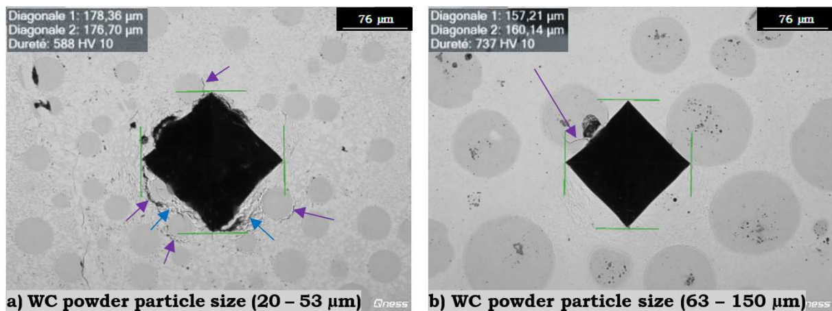
Figure 11: Hardness imprints on the polished surface of coatings deposited by LC from the mixture of the NiCrBSi matrix with 60 wt% of WC carbide powder with different particle sizes a) 20 - 53 \mu\text{m} and b) 63 - 150 \mu\text{m}
