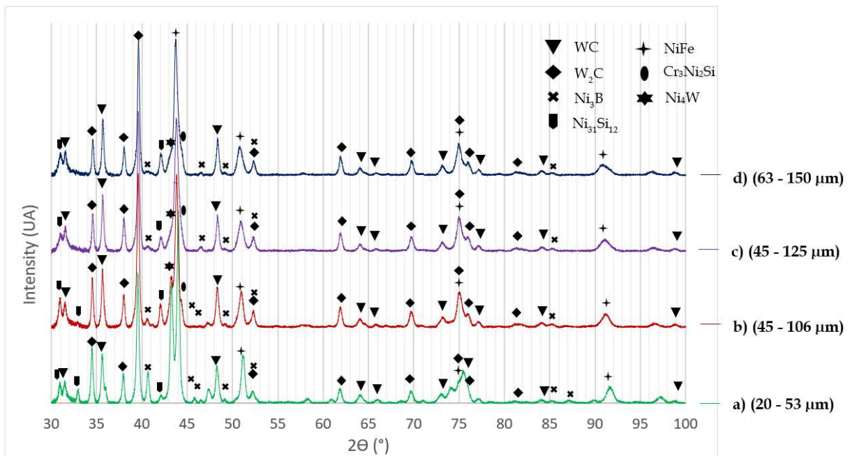
Figure 8: Diffractograms of coatings deposited by LC from powder mixtures with the NiCrBSi matrix (11 wt% Cr) reinforced with 60 wt% of WC tungsten carbide powder with different particle sizes.
