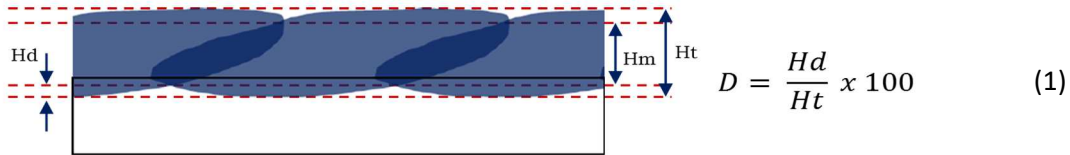
Figure 3: Evaluation method of the substrate dilution for coatings deposited by LC with: D = dilution rate (%), H_t = total thickness ( \mu\text{m} ), H_m = minimum coating thickness ( \mu\text{m} ) and H_d = dilution thickness of the substrate ( \mu\text{m} ) [11].
