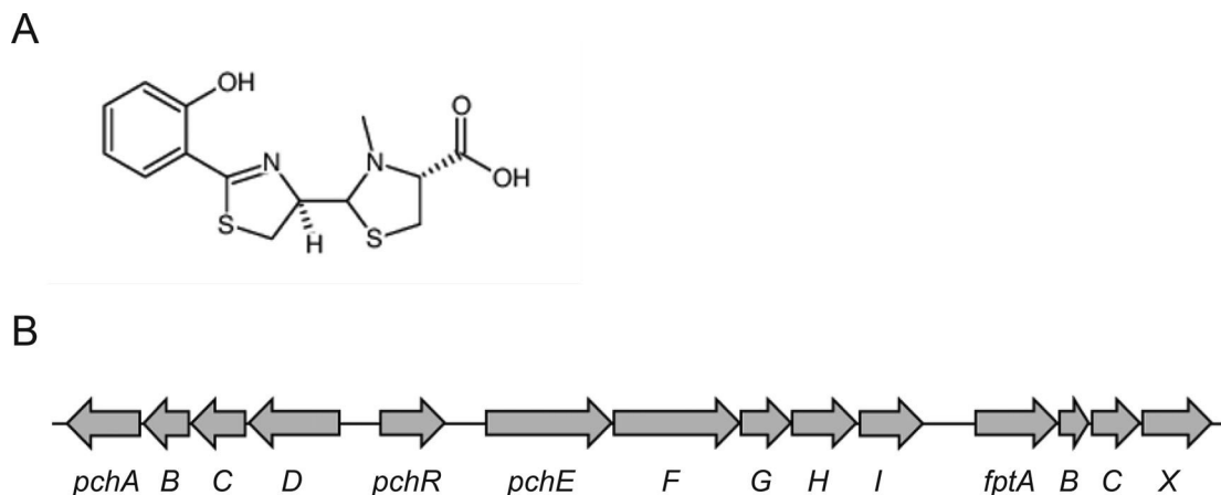
Fig. 1. Pyochelin structure and locus from P. aeruginosa . (A) Chemical structure of PCH. (B) Schematic map of the PCH locus. pchABCDEF are genes involved in PCH biosynthesis, pchR encodes a transcriptional regulator, fptA the PCH-Fe outer membrane transporter, fptX the PCH-Fe inner membrane permease and pchH , pchI , fptB and fptC proteins of unknown function.
