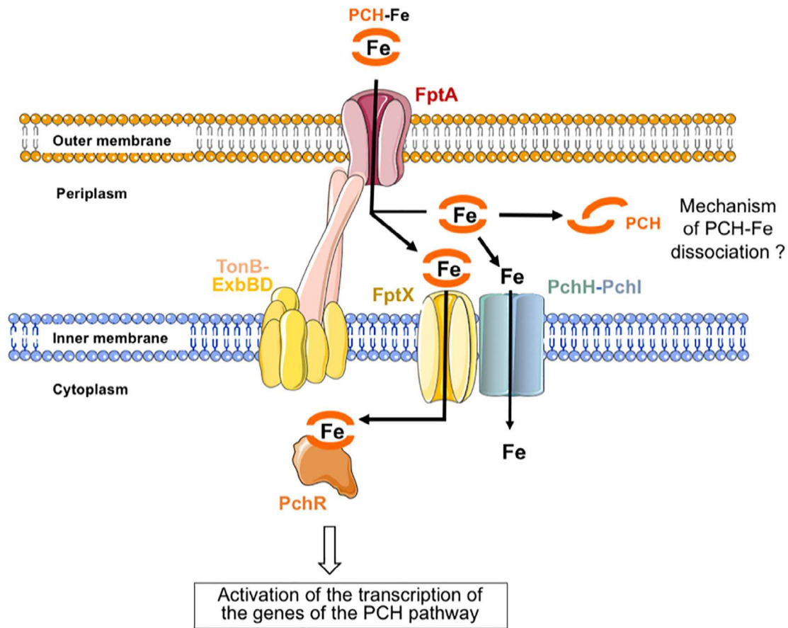
Fig. 6. Model of the PCH-Fe uptake pathway in P. aeruginosa . The PCH-Fe complexes are recognized by the outer membrane transporter FptA, allowing their translocation into the bacterial periplasm. A first fraction is transported further into the cytoplasm by FptX to interact with PchR, while a second fraction of the PCH-Fe complexes would undergo a dissociation in the bacterial periplasm by an unknown mechanism and the free iron transported further across the inner membrane into the bacterial cytoplasm by PchHl.
