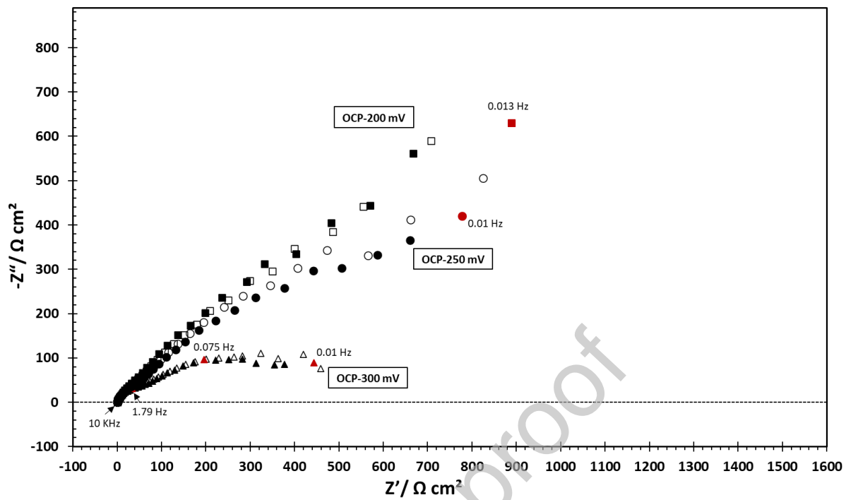
Figure 11. Nyquist plot at different OCP – 200 mV, OCP – 250 mV and OCP – 300 mV.
