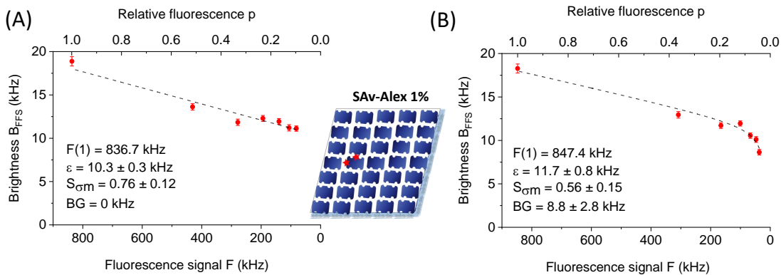
Figure 4: Characteristic brightness decay versus the fluorescence signal for a SAV layer prepared with 1% dilution of SAV-Alex. (A) Example without background (i.e. fixed to 0), showing the linear decay and the fit (dashed black line) with the \epsilon and S_{\sigma m} outputs corresponding to the measured (red) points; the errors bars are the standard errors of the mean calculated from the 8 \times 8 sub-images; (B) In presence of background, the corresponding parameter, BG , can be fitted (it represents about 1% the initial fluorescence signal, F(1) ), while the other outputs, \epsilon and S_{\sigma m} , are consistent with the results of the background-free case.
