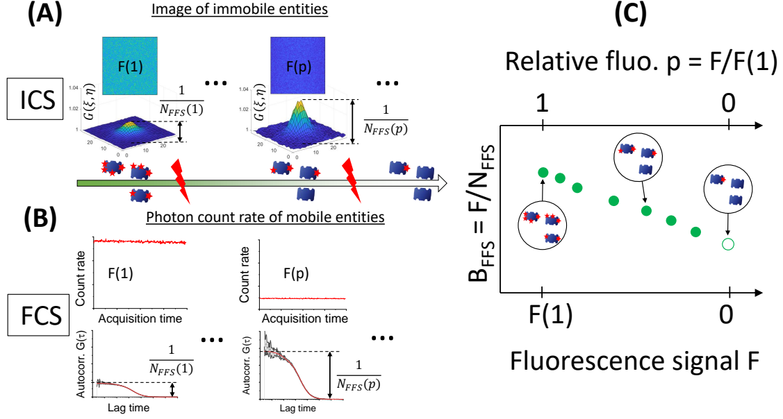
Figure 1: Principle of a pbFFS experiment, where a series of measurement phases, ICS or FCS, are alternated with photobleaching phases (red flashes). The latter induce a decrease of the number of unbleached fluorescent labels, as shown along the graded green central arrow, that is a decrease of the fluorescence signal, F , observed during the measurement phases, corresponding to the mean image intensity in ICS with immobilized fluorescent entities (A), or to the mean photon count rate for FCS with mobile fluorescent entities (B). Correspondingly, the number of entities measured by FFS, N_{FFS} , decreases as can be seen by the increased amplitude of the spatial autocorrelation in ICS, G(\xi, \eta) , or temporal autocorrelation in FCS, G(\tau) . Part (C) shows that the brightness measured during the successive phases, defined as B_{FFS} = F/N_{FFS} , plotted vs the fluorescence signal, monotonously decreases upon photobleaching and tends towards that of a single fluorescent label.
