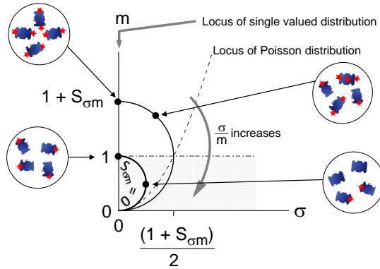
Figure 2: Geometrical representation of the relation between the mean, m , and the standard deviation, \sigma , of the initial number of fluorescent labels per entity. For a given measured slope, S_{\sigma m} , the support of the (\sigma, m) points is a half circle of diameter 1 + S_{\sigma m} that always crosses the (0, 0) point; the coefficient of variation of the distribution of the number of fluorescent labels, \frac{\sigma}{m} , continuously increases from the top to the base of the half-circle. Single-valued distributions correspond to discrete points located on the vertical axis ( \sigma = 0 ), as exemplified for 1 and 2 fluorescent labels. The smallest circle of diameter 1 ( S_{\sigma m} = 0 ) corresponds to a mixture of entities bearing either no fluorescent label or exactly one, as depicted at the bottom right. If all molecules bear at least one fluorescent label, for instance a mixture of 1, 2 and 3 fluorescent labels, the (\sigma, m) solutions are located in the upper half space above the dashed-dotted line m = 1 . Note that in the case of a Poisson distribution, any given slope S_{\sigma m} corresponds to a unique point (\sigma, m) located at the intersection of the m = \sigma^2 curve (dashed line) and of the half circle of diameter 1 + S_{\sigma m} (see text).
