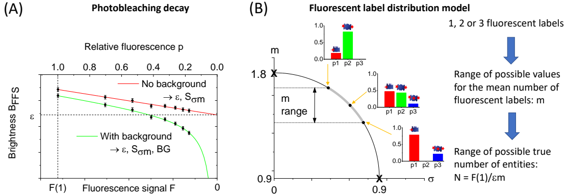
Figure 3: Schematics of the implementation of the brightness decay analysis: (A) Upon photobleaching, the brightness, B_{FFS} , decreases linearly versus the fluorescence signal, F or p (red solid line), thus providing the output parameters \epsilon and S_{\sigma m} ; in case of background (green solid line) an additional parameter, BG , can be estimated by fitting the decay (see text for details). (B) By combining the relation between m and \sigma corresponding to the measured value of S_{\sigma m} and the constraints deriving from three non-nil probabilities ( p_1 , p_2 and p_3 for 1, 2 or 3 fluorescent labels), the possible m values are restricted to a limited range; three examples of distributions of probabilities corresponding to the minimum, maximum and central values of m are depicted for S_{\sigma m} = 0.8 . Finally, this analysis provides a value of the mean number of fluorescent labels, m , which combined with the initial fluorescence signal, F(1) and the parameter \epsilon , leads to an estimation of the true number of entities, N .
