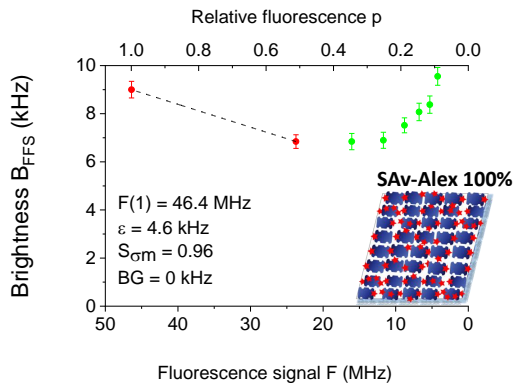
Figure 5: Example of the dramatic consequence, for the brightness decay, of the fluorescence quenching between Alexa555 fluorophores of a streptavidin layer prepared with 100% of SAv-Alex. Note that the single fluorescent label brightness, \epsilon , is more than twice smaller than its value at high dilution (see Fig. 4), while the S_{\sigma m} parameter, estimated from the 2 first points, stays consistent.
