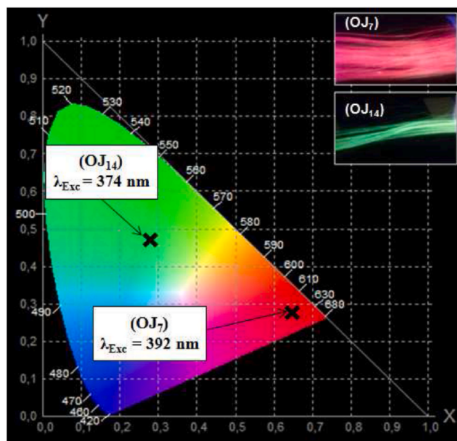
Fig. 10. CIE color coordinates of PGFs samples on CIE 1931 chromaticity diagram upon excitation at 392 nm (OJ 7 ) and 374 nm (OJ 14 ).
