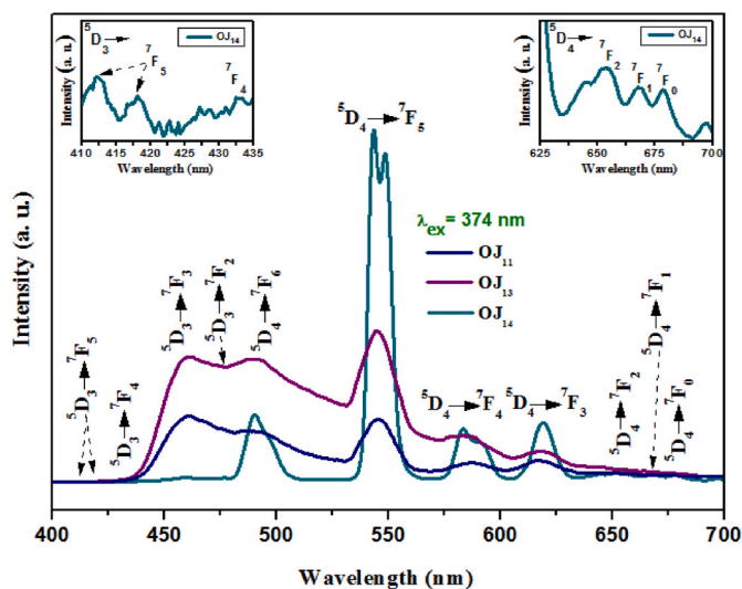
Fig. 9. Emission spectra of Tb 3+ -doped PGFs samples under 374 nm excitation at 300 K.
