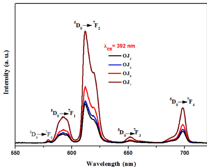
Fig. 8. Emission spectra of Eu 3+ -doped PGFs samples under 392 nm excitation at 300 K.
