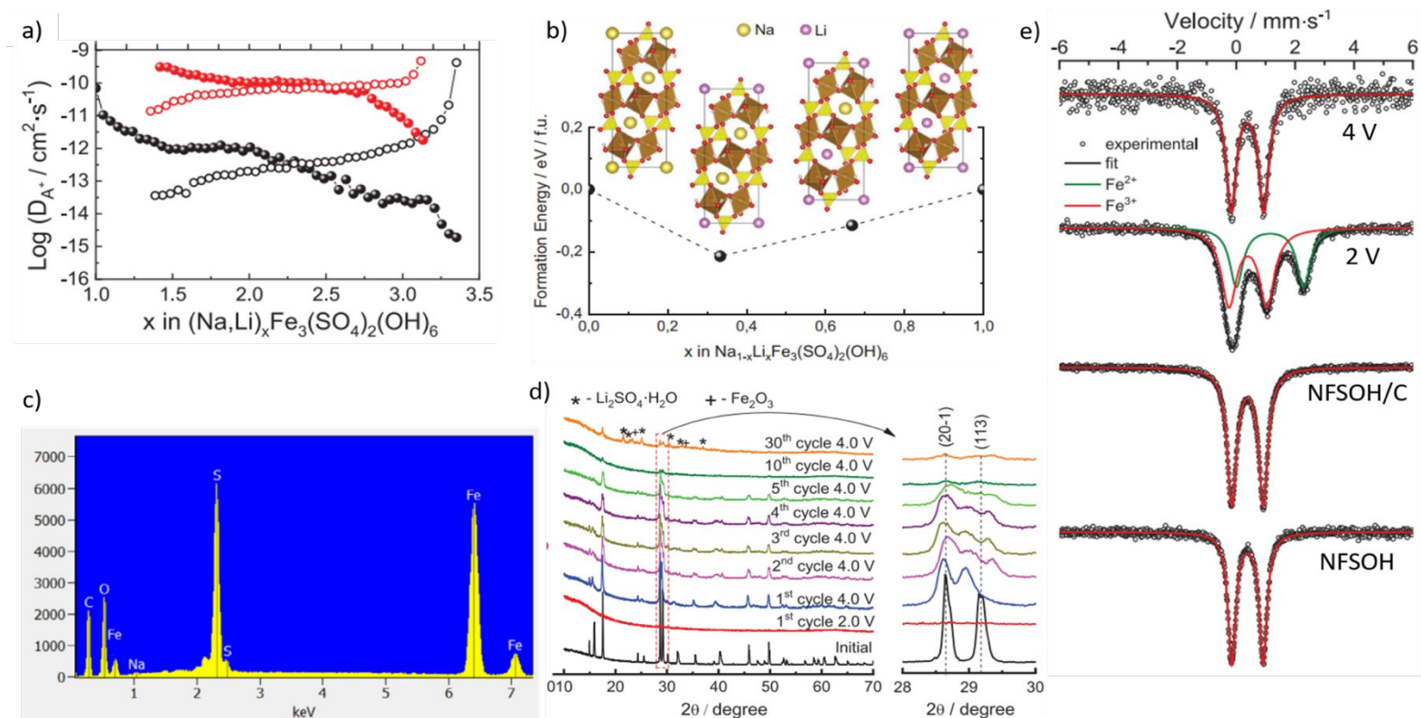
Figure 8. (a) Coefficient of diffusion D_{A^+} ( A^+=\text{Li}^+, \text{Na}^+ ) calculated from GITT plot at different value of x [(\text{Na,Li})_x\text{Fe}_3(\text{SO}_4)_2(\text{OH})_6] during 1 st (black sphere/circle) and 2 nd cycle (red sphere/circle). (b) Formation energy estimated using DFT calculations for different values of x in \text{Na}_{1-x}\text{Li}_x\text{Fe}_3(\text{SO}_4)_2(\text{OH})_6 . (c) Evidence of substitution of structural \text{Na}^+ with \text{Li}^+ is observed on comparison of EDS spectra of pristine NFSOH/C composite (see reference) and after 10 th charge. Minor peak at \sim 1 keV indicate low amount of Na atoms in NFSOH crystal structure. (d) Ex situ XRD pattern comparison during 1 st cycle, 2 nd charge, 3 rd charge, 4 th charge, 10 th charge and 30 th charge. (e) ^{57}\text{Fe} Mössbauer spectra of pristine natrojarosite, NFSOH ( \text{NaFe}_3(\text{SO}_4)_2(\text{OH})_6 ), NFSOH/C composite, NFSOH/C composite at 1 st discharge (2 V) and NFSOH/C composite at 1 st charge (4 V). A constant isomer shift value of 0.38 \text{ mm} \cdot \text{s}^{-1} is reported across four samples. Reproduced with permission. 106 Copyright 2020, Elsevier Ltd.
