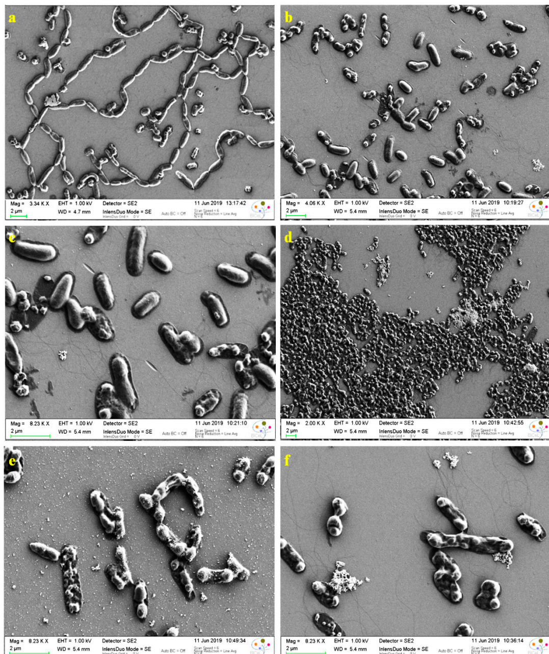
Figure 9. SEM images of E. coli : (a) control and incubated with CuS-BSA/lysozyme nanoparticles at a concentration of 100 \mu\text{g/mL}^{-1} (b,c) without and (d–f) under 980 \text{ nm} ( 1 \text{ W cm}^{-2} ) irradiation.
