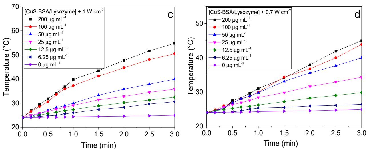
Figure 4. Photothermal heating curves of (a,b) CuS-BSA and (c,d) CuS-BSA/lysozyme at various concentrations in 0.01 \text{ mol L}^{-1} PBS under NIR illumination (980 nm) under a continuous wave laser irradiation at different power densities for 3 min.
