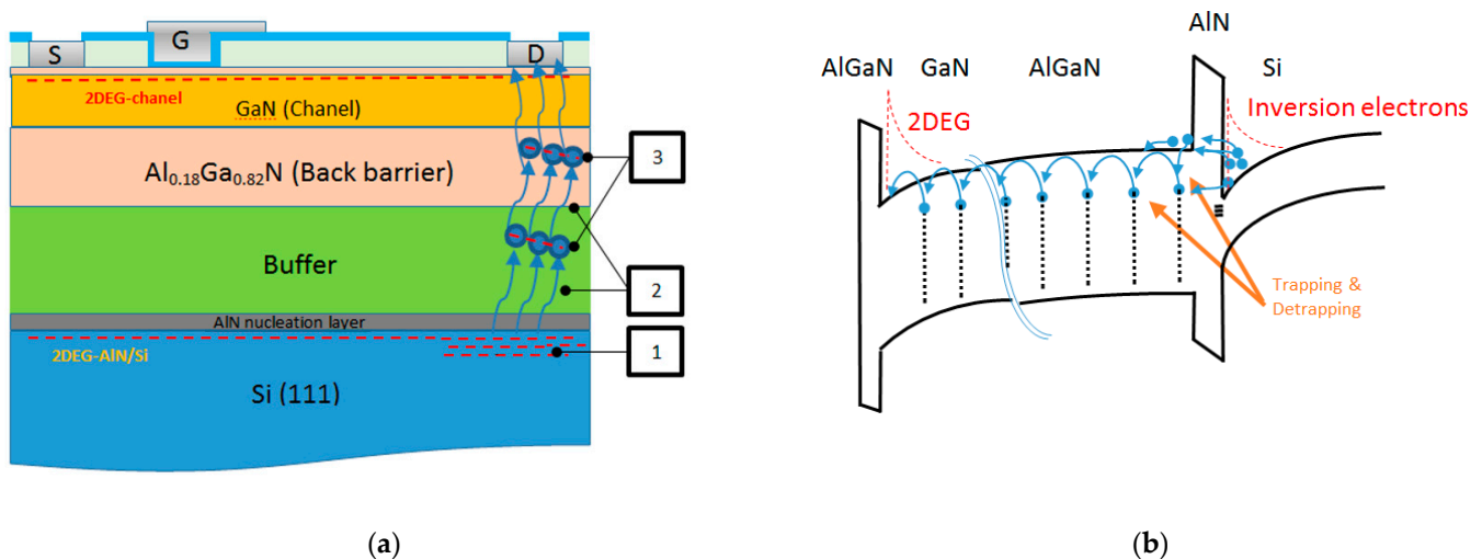
Figure 6. Physical mechanisms responsible for the vertical leakage: (a) Leakage current from AlN/Si interface through the AlN and buffer layer to the drain electrode (1) 2DEG at the AlN/Si interface constitutes the main source of electrons at high leakage currents. (2) Electrons are injected into the transition layers. (3) The current is limited by trapping of electron into acceptor states (SCLC). (b) The mechanisms of electron injection across the AlN barrier.
