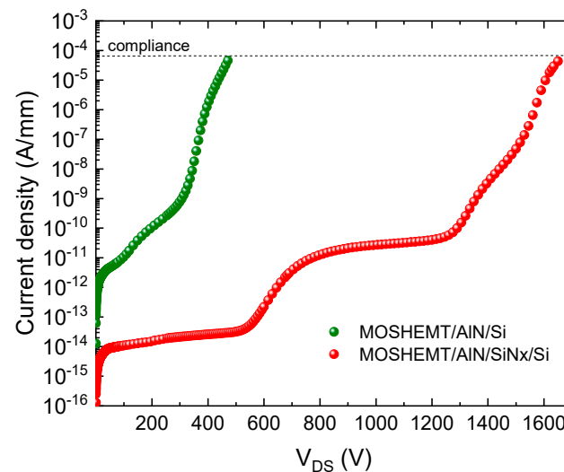
Figure 9. Drain current Vs drain voltage of MOS-HEMT with ( V_{BD} = 1500 V) and without SiN x interlayer ( V_{BD} = 500 V).
