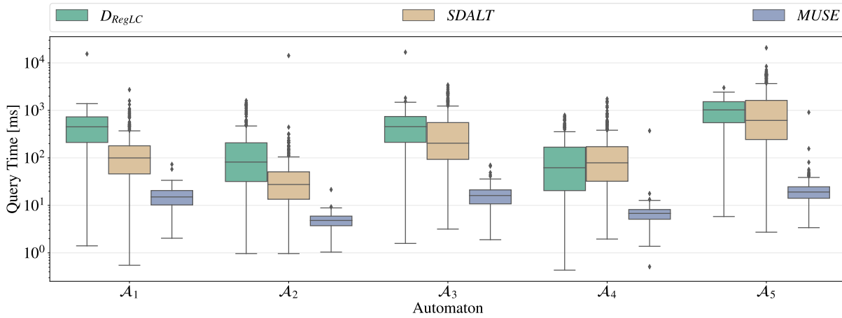
Figure 12 Query times distribution of D_{RegLC} , SDALT , and the 300-based partition size MUSE for each automaton on the Ile-de-France region graph.
