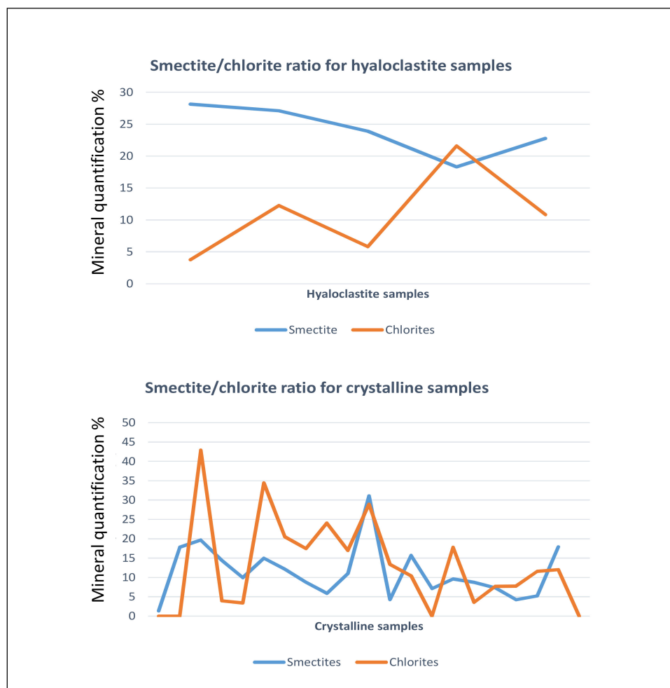
Figure 14. Chlorite and smectite quantification (volume percentage) from XRD measurements. X axis: analyzed samples (5 samples for hyaloclastites, 21 samples for crystalline rocks).
