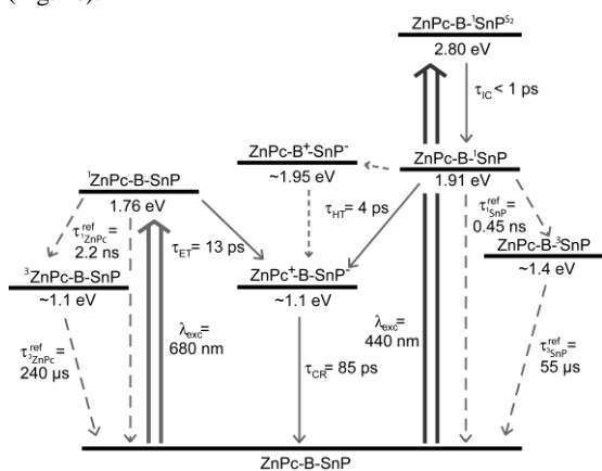
Fig. 3. Summary of the relevant states and transitions (in benzonitrile 17 ).
