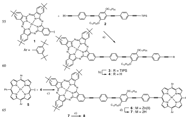
Scheme 1. Synthetic route to the dyads 6-8 . Reagents and conditions : a) piperidine, Pd 2 dba 3 -CHCl 3 , AsPh 3 , 40°C, 15h (43%); b) Bu 4 NF, THF (100%); c) THF, Et 3 N, Pd 2 dba 3 -CHCl 3 , AsPh 3 , 60°C, 15h (33%); d) HCl, CH 2 Cl 2 (91%); e) pyridine, SnCl 2 -2H 2 O, 185°C, 3h (83%).
