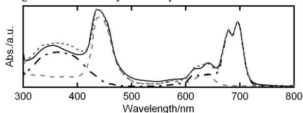
Fig. 1. Overlay of UV-Vis. spectra of the dyad 8 (straight line) along with those of 3 (dashed-dotted line) and 12 (dashed line) recorded in benzonitrile.
