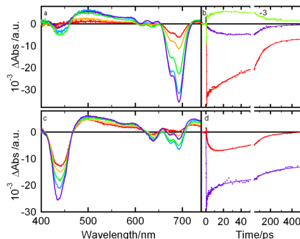
Fig. 2. Transient absorption of dyad 8 in benzonitrile. The plot in (a) corresponds to excitation at 680 nm and (c) to an excitation at 440 nm. The delay times are 1 ps (purple), 10 ps (blue), 50 ps (green), 200 ps (orange) and 1000 ps (red). Plots (b) and (d) correspond to the kinetic traces at 440 nm (purple) and 690 nm (red) and 730 nm (green, multiplied with 3 for clarity) for the respective excitations.
