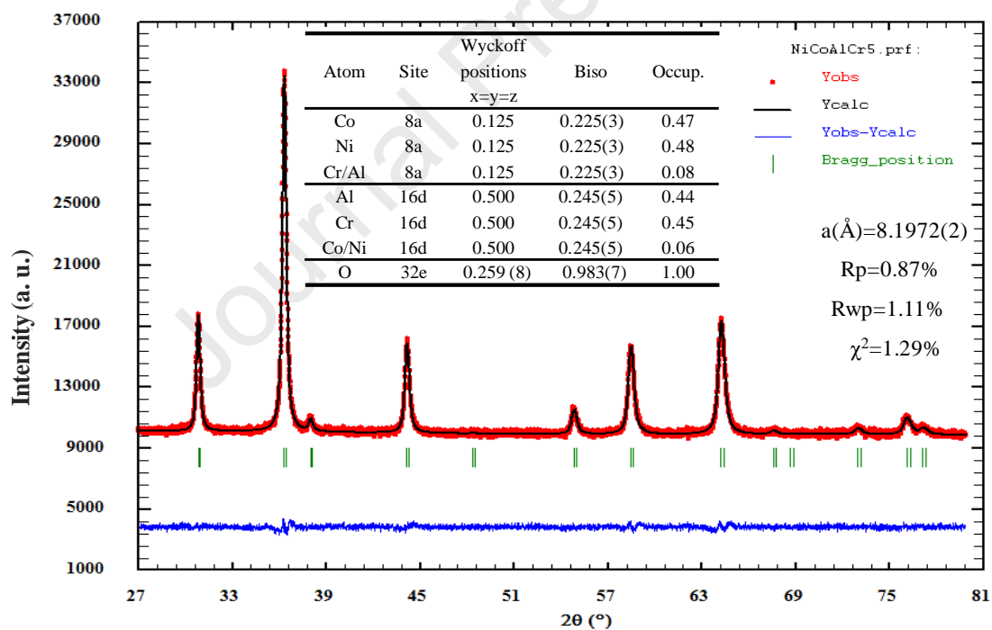
Fig. 4. Rietveld refinement of XRD pattern of \text{Ni}_{0.5}\text{Co}_{0.5}\text{CrAlO}_4 sample.
