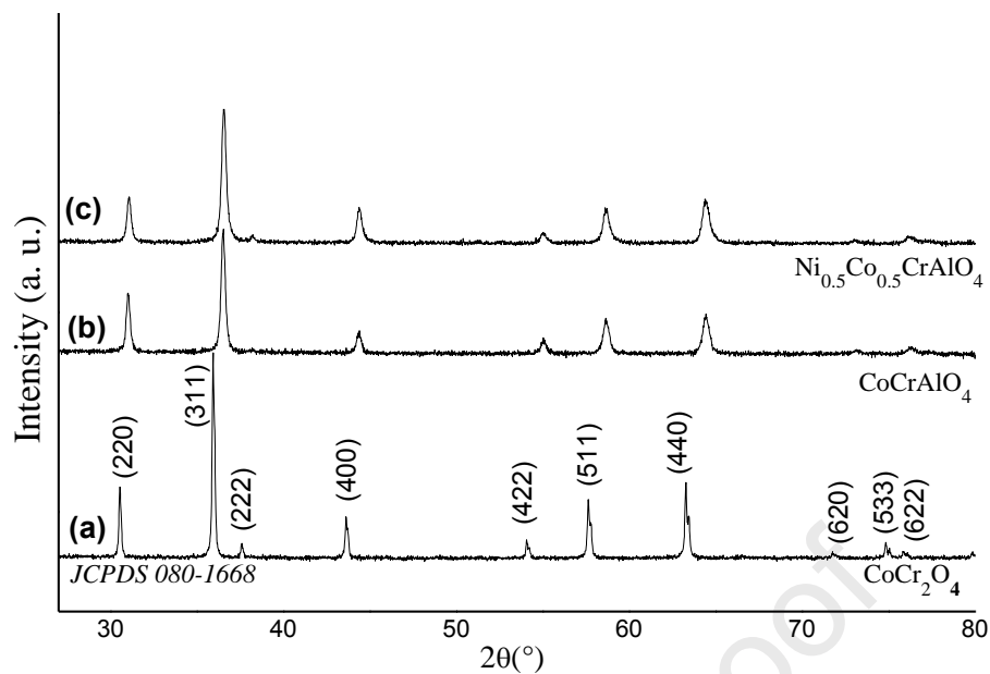
Fig. 3. X-ray diffraction patterns of \text{CoCr}_2\text{O}_4 and substituted spinels.
