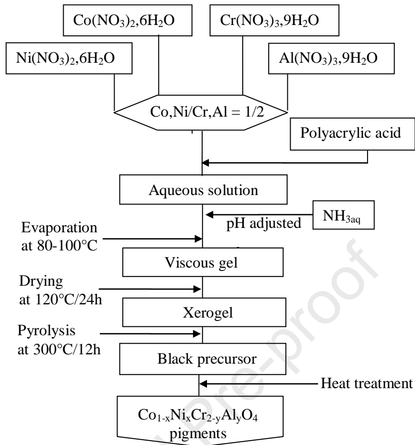
Fig. 1. Flowchart for the preparation of \text{Co}_{1-x}\text{Ni}_x\text{Cr}_{2-y}\text{Al}_y\text{O}_4 ( 0 \leq x \leq 1 , 0 \leq y \leq 2 ) powdered pigments.
