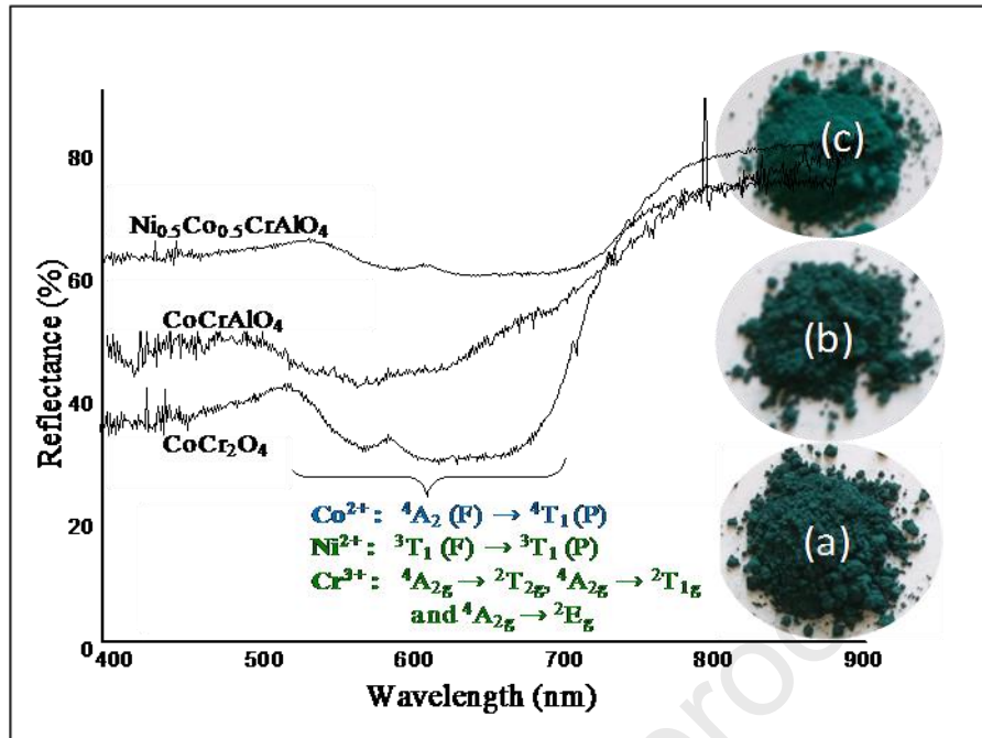
Fig. 5. Shades of the green colour and diffuse reflectance spectra of (a): \text{CoCr}_2\text{O}_4 , (b): \text{CoCrAlO}_4 and (c): \text{Ni}_{0.5}\text{Co}_{0.5}\text{CrAlO}_4 powders.
