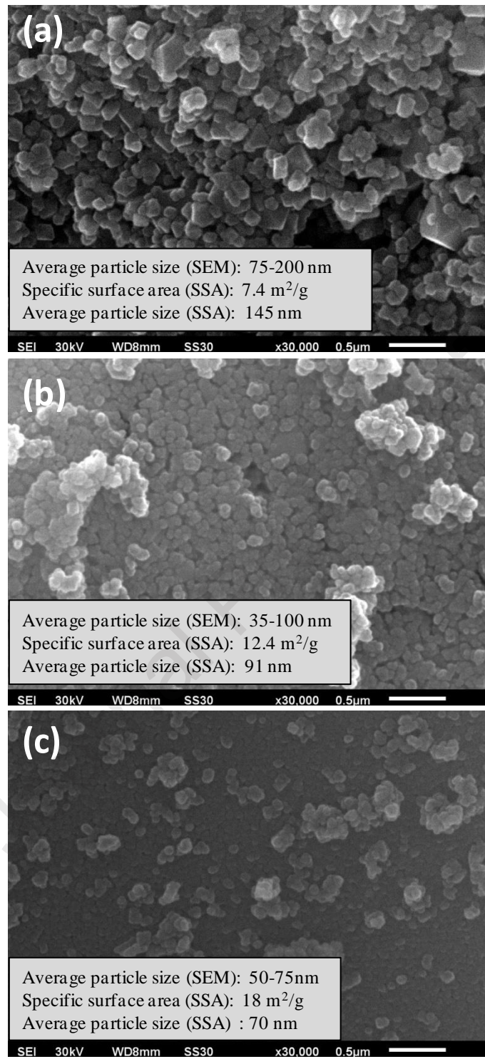
Fig. 6. SEM micrographs and estimated grain sizes of (a): \text{CoCr}_2\text{O}_4 , (b): \text{CoCrAlO}_4 (c): \text{Ni}_{0.5}\text{Co}_{0.5}\text{CrAlO}_4 powders.
