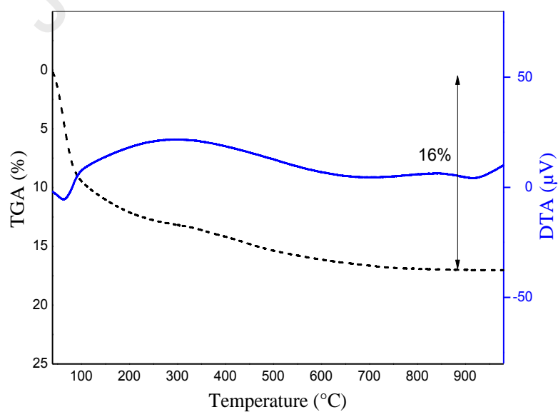
Fig. 2. TG-DTA analysis of dried gel of \text{CoCr}_2\text{O}_4 precursor.
