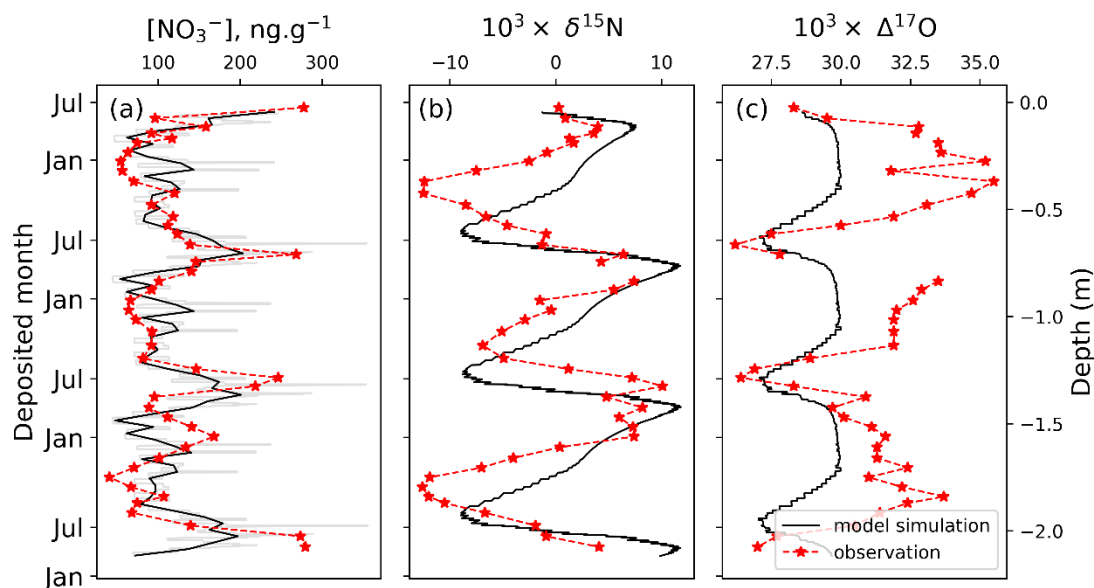
Figure 1. Comparison between the observed and modeled snowpack nitrate profiles. We used same snow accumulation rate for each year in the model. The measured minimum \Delta^{17}\text{O}(\text{NO}_3^-) is used as indicator of June-July when local photochemistry is most active.
