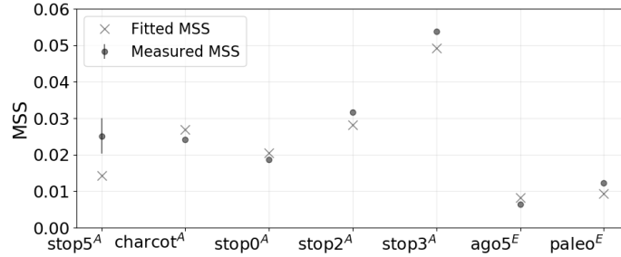
Figure 11: Measured (points) and fitted (crosses) Mean Square Slopes of the surface (MSS). Standard deviation at stop5 A represents the measured variability between the two nearby sampled areas.
