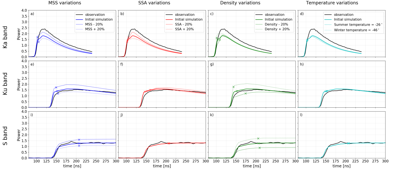
Figure 10: Waveform variations at stop2 A with MSS variations of \pm 20\% in simulations (first column); with SSA variations of \pm 20\% (second column); with density variations of \pm 20\% (third column); with temperature variations from the mean summer temperature (December and January) to the mean winter temperature (June and July) (fourth column). The slope of the stop2 A site is of 0.15^\circ . Results are given for the Ka band of SARAL-Altika (first row), the Ku band of ENVISAT (second row) and the S band of ENVISAT (third row). Simulated waveform maximums are indicated with crosses.
