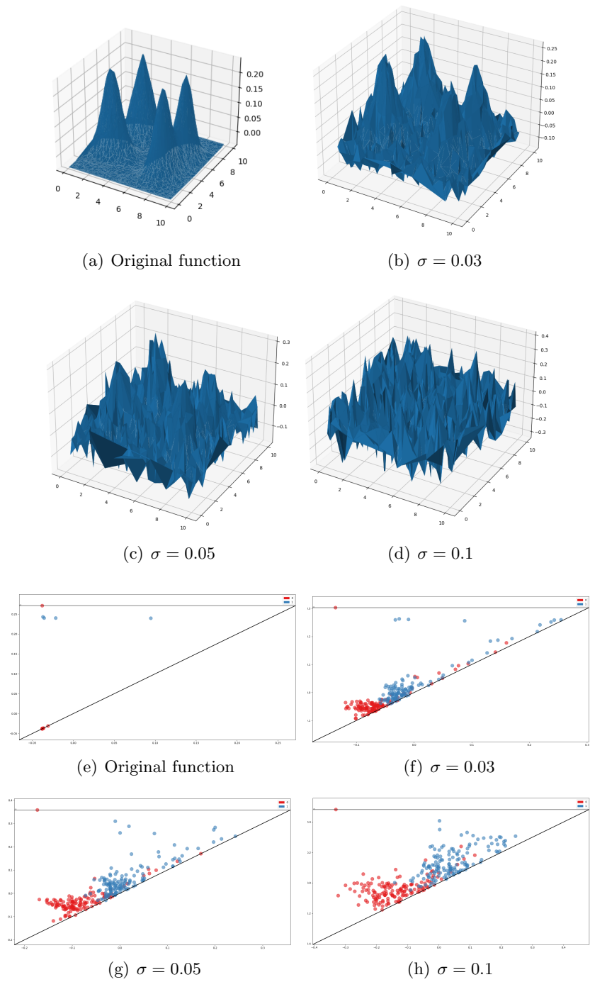
Figure 3: Influence of noise on persistence diagrams.
