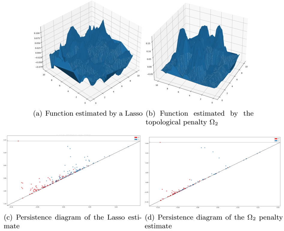
Figure 7: Reconstruction of the sum of four Gaussians.
