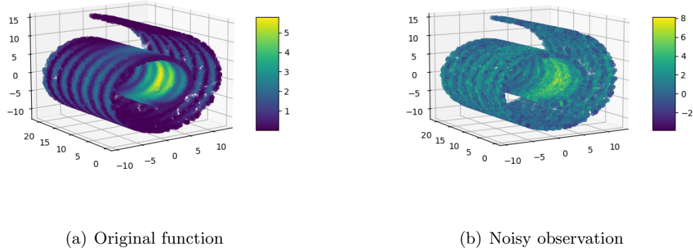
Figure 9: Regression function on a Swiss roll
