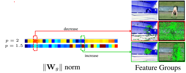
Figure 9: Sparse feature weighting illustration. On the left, \|W_g\|_2 are displayed, for p = 2 or 1.5 . On the right, features corresponding to W_g groups are shown.
