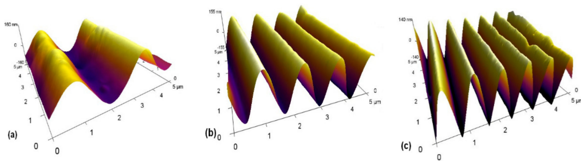
Figure 7. Three-dimensional AFM images of the SRG, inscribed in the thin film sample with NP concentration C = 10\% and recording angles (a) 2\theta = 10^\circ , (b) 2\theta = 20^\circ , and (c) 2\theta = 30^\circ .
