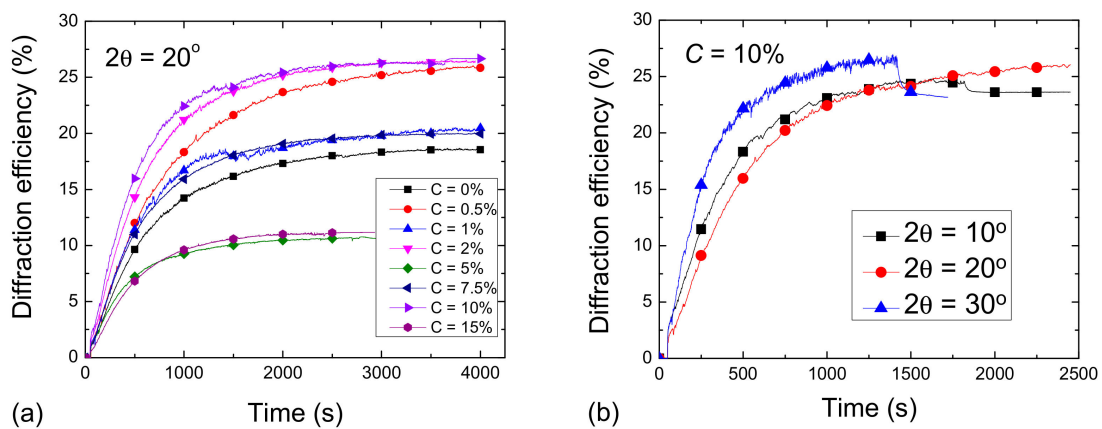
Figure 4. Kinetics of the diffraction efficiency in the +1 order during the holographic recording: (a) for recording angle 2\theta = 20^\circ and all samples with C = 0\text{--}15\% , (b) for concentration of the goethite nanorods C = 10\% and recording angles 2\theta = 10^\circ, 20^\circ , and 30^\circ (symbols are plotted in (a) at every 500 and in (b) at every 250 data points to distinguish the curves).
