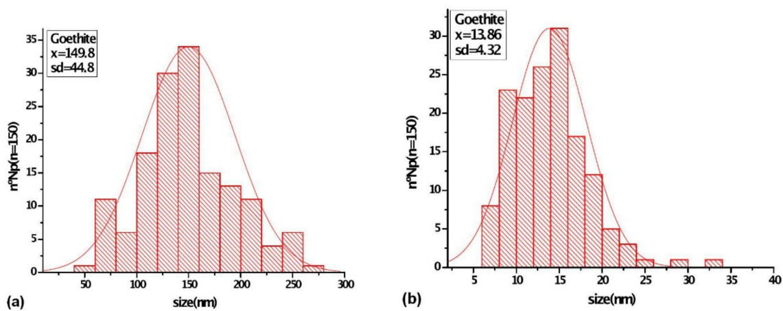
Figure 3. Histogram of the goethite nanorods size distribution based on n = 150 nanoparticles evaluated. (a) NP length distribution; (b) NP width distribution.
