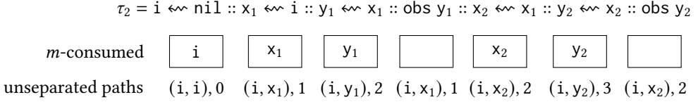
Fig. 7. A depiction of the abstract graphs of the program in Figure 3, with the same trace as Figure 6. At each operation, we depict the m -consumed abstract graph, which is a set of nodes that have been introduced but not consumed. Because this set is empty at the end of any iteration, the program satisfies the m -consumed semantic property. The unseparated paths abstract graph is a mapping, for each unseparated path in the graph, from its pair of endpoints to its length. We depict the longest path residing in the mapping. After each iteration, this longest path continues to lengthen, so the program does not satisfy the unseparated paths semantic property.
