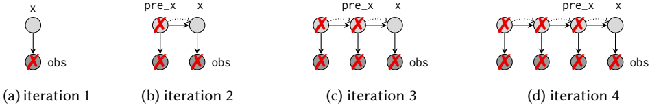
Fig. 2. The evolution of the delayed sampling graph for the hidden Markov model in Figure 1 (hmm) as implemented by Baudart et al. [2020]. Each node denotes either a value (dark gray) or a distribution (light gray). A plain arrow denotes a dependency in the underlying Bayesian network. A dotted arrow denotes a pointer in the implementation of the delayed sampling graph. Each label indicates the program variable that corresponds to a node. An X on a node denotes that the node is not reachable from the program state.
