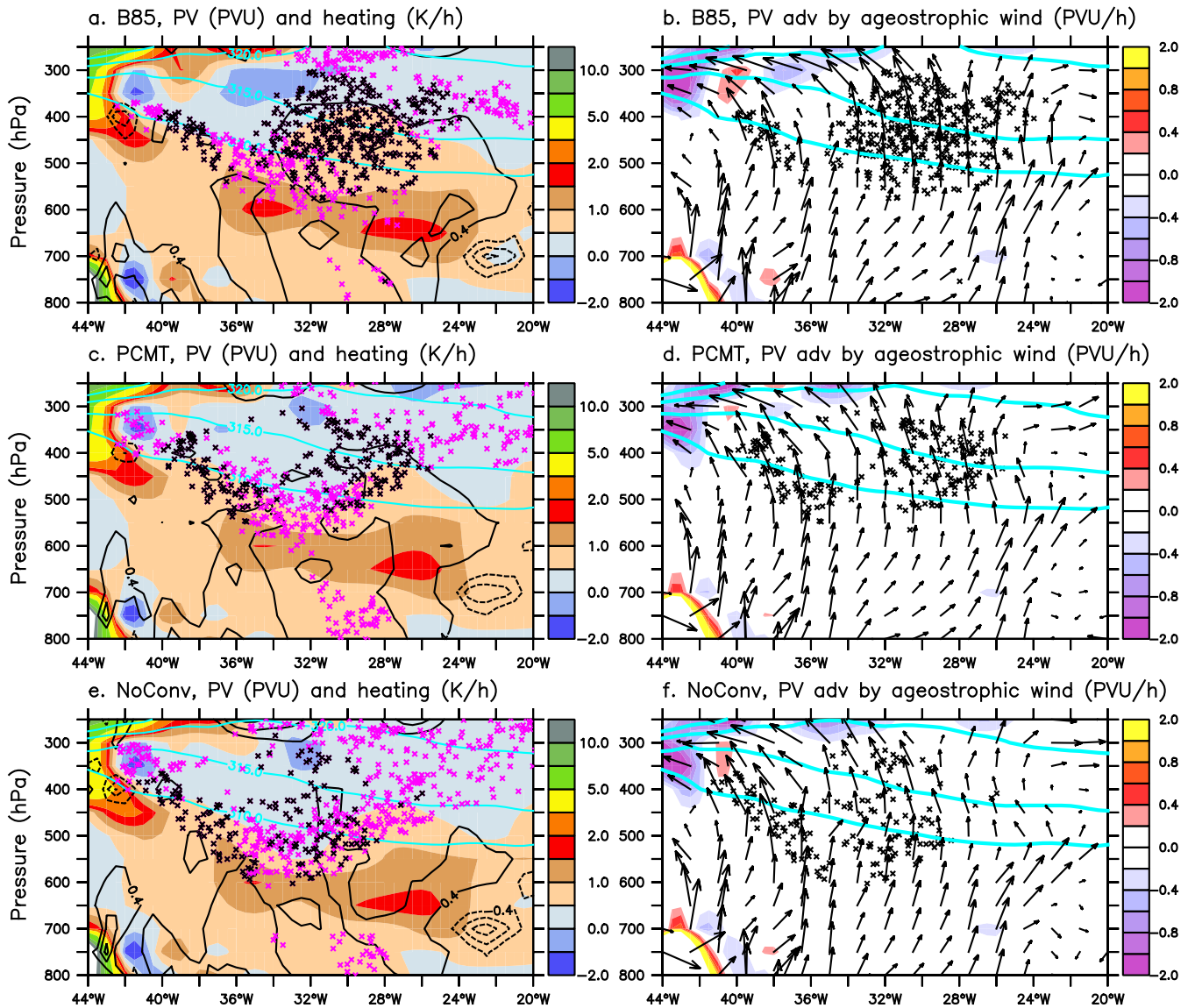
Figure 7. (Left panels) Latitudinally-averaged ( 63^{\circ}\text{N} - 65^{\circ}\text{N} ) PV (shadings; units: PVU), heating rate (black contours; int: 0.4\text{ K h}^{-1} ), potential temperature (light blue contours for 310, 315, 320 and 325 K) and WCB trajectories satisfying 25 hPa ascent in 2 hours (black crosses) and the other WCB trajectories (purple crosses) and located in the same latitudinal band at 12 UTC 2 October for (a) B85, (c) PCMT and (e) NoConv simulations. (Right panels) Latitudinally-averaged ( 63^{\circ}\text{N} - 65^{\circ}\text{N} ) PV advection by the zonal and vertical components of the ageostrophic wind (shadings; units: \text{PVU h}^{-1} ), and the associated ageostrophic wind vectors (black arrows). The light blue contours represent potential temperature as in left panels. The ageostrophic wind vectors are represented by multiplying respectively the zonal and vertical components by the distances occupied by 1 meter in longitude and 1 Pa in pressure on the diagram.
