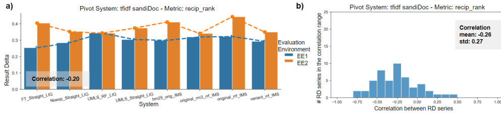
Figure 4. a) Result Delta comparison between two EEs using the pivot tfidf_sandiDoc and the recip_rank metric; b) distribution of the correlation of 50 pairs of EEs using a pivot and a metric.
