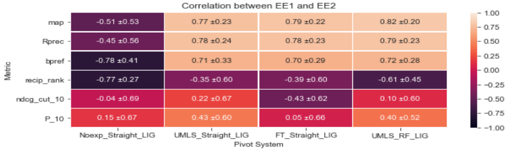
Figure 6. Correlation (mean and std. dev.) between result deltas in two evaluation environments considering only LIG’s systems. Systems are listed in decreasing MAP value (left to right) according to the official results.
