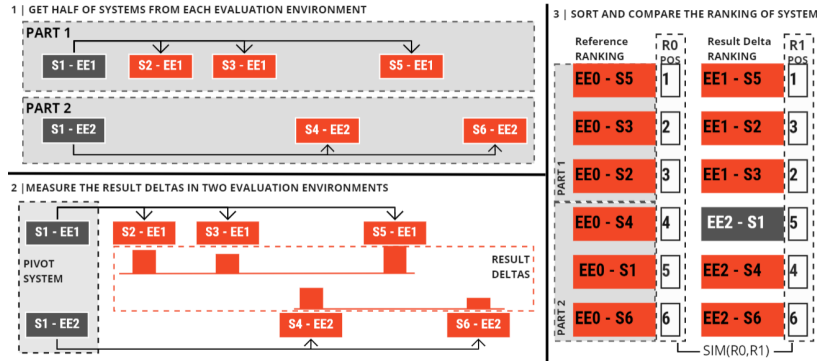
Figure 3. Method to create a ranking of systems evaluated in different EEs using result deltas.
