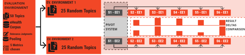
Figure 2. Method to measure and compare the result deltas of two evaluation environments using pivot S1 .
