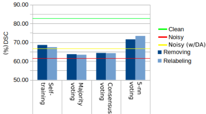
Figure 6: DSC on Syncracks’s clean validation data using corrected labels.
