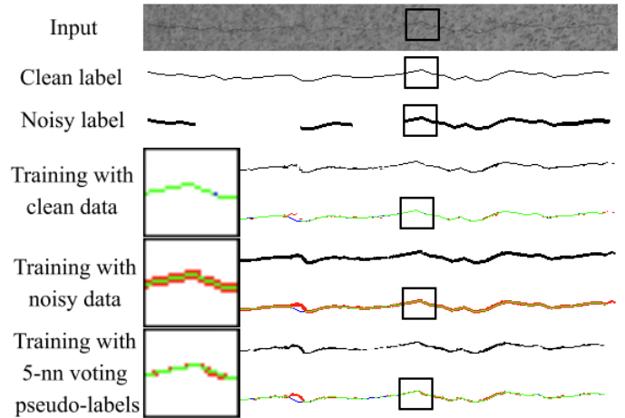
Figure 7: Prediction comparison of U-VGG19 on Syncracks. In the last three rows, black-lines show predictions and colored lines show the comparison with the clean label (the color code is the same as in Fig. 4).
