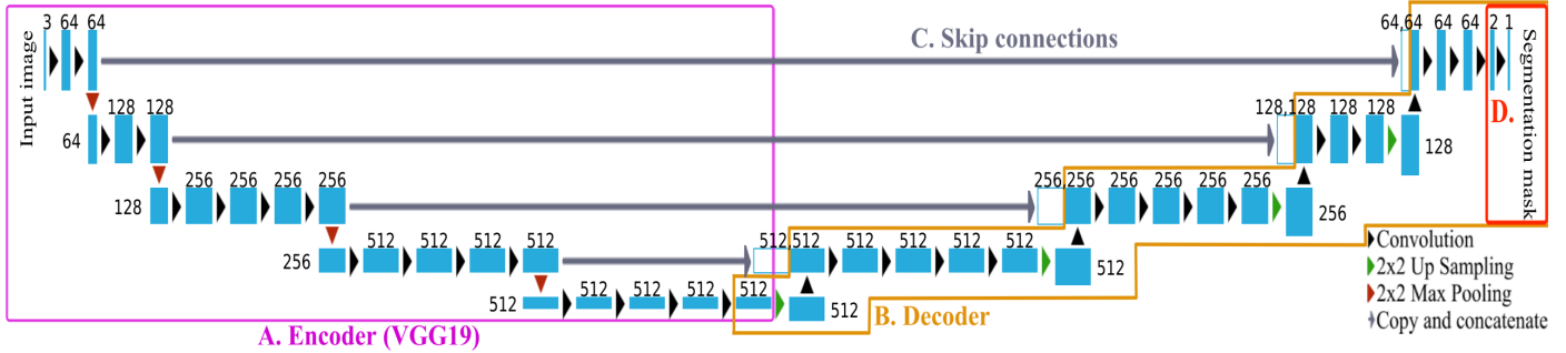
Figure 3: U-VGG19 architecture.
