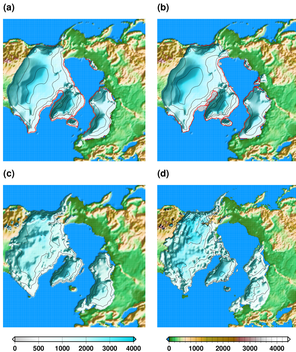
Figure 2. Surface elevation above contemporaneous sea level: (a) after the glacial spin-up, (b) in the reference deglaciation experiment DGL at 21 ka, (c) in the GLAC-1D reconstruction and (d) in the ICE-6G_C reconstruction. The colour scale is different for ice-free and ice-covered regions. The simulated ice sheet grounding line is represented by the red line, while the black lines represent isocontours of ice sheet surface elevation (separated by 1000 m).
