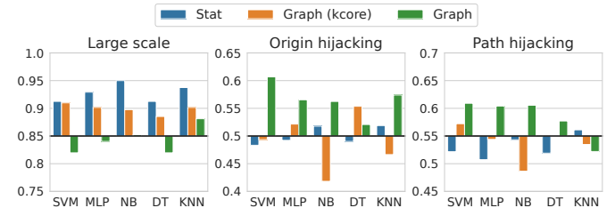
Fig. 4. Accuracy (see eq. 2) of ML models
