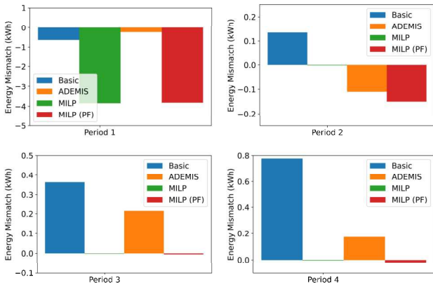
Fig. 5. Total energy mismatch comparison for each period
