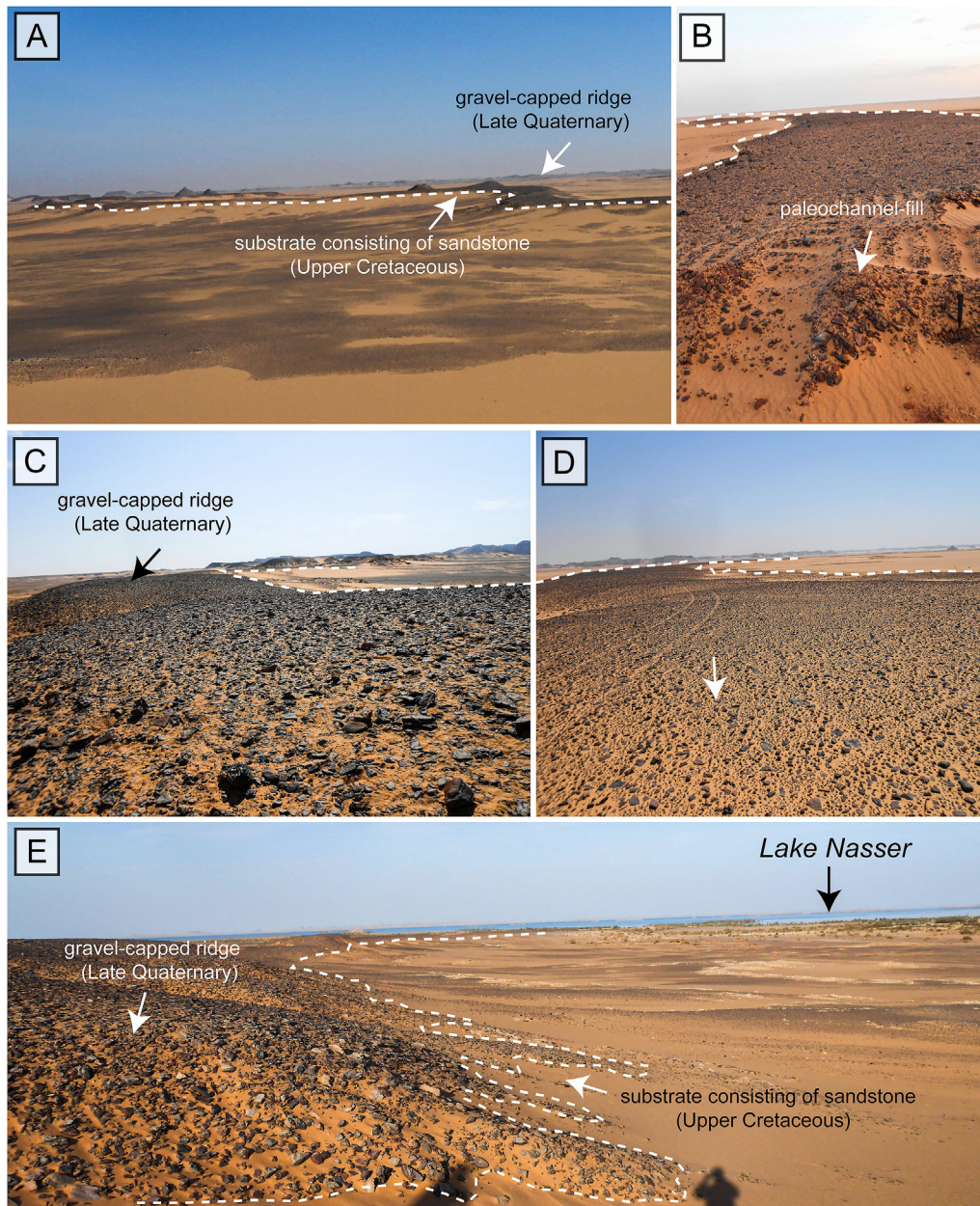
Fig. 3. Field photographs of ridges preserving a former rivers; (A) Gabal Hamam, (B) Arqin I, (C) Gabal Hamam I, (D) Gabal Masmas, and (E) Gabal El Sadd. The ridges typically comprise two stratigraphic units; the upper unit is gravel deposited during the Late Quaternary, and the lower unit consists of sandstone accumulated during the Upper Cretaceous epoch.
