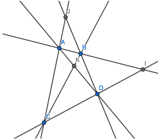
Fig. 3. An illustration of the new form of Pasch's axiom used to deal with symmetries
