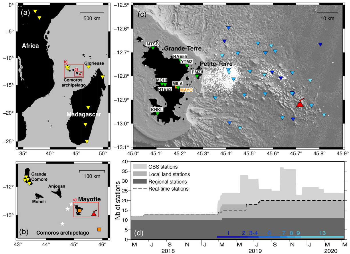
Figure 1. Maps of seismicological land stations and Ocean Bottom Seismometers (OBSs) used in this study with the red volcano symbol representing the location of the new volcanic edifice (Feuillet et al. 2021). (a) Map showing the regional stations contributing to the monitoring (yellow inverted triangles). Red rectangles highlights the Comoros archipelago area shown in (b) and the Mayotte area shown in (c). (b) Map of the Comoros archipelago showing the temporary stations used for previously-developed velocity profiles (orange squares), historical M > 5.0 earthquakes close to Mayotte (white stars) and the Karthala seismic network (yellow inverted triangles). (c) Map of the local land stations (green inverted triangles, most of them installed in 2019) and all OBSs deployed between February 2019 and May 2020 [blue inverted triangles, the blue hue depends on the MAYOBS deployment timing as seen in (d)]. The MAYOBS station (orange square) is the temporary station used by Dofal et al. (2018) receiver function study. The white dots represent the 5000 manually relocated earthquakes. (d) Time evolution of the number of recording stations since the onset of the crisis. All regional stations (dark grey) are available in real-time. Local stations (added to the regional stations; in grey)—significantly increased in number in 2019. The number of OBSs (added to the local and regional stations; in light grey) varies over time depending on the MAYOBS deployment period (blue scale on bottom right numerated as the MAYOBS oceanographic campaigns that recovered them). The dashed line represents the evolution in time of the number of real-time stations.
