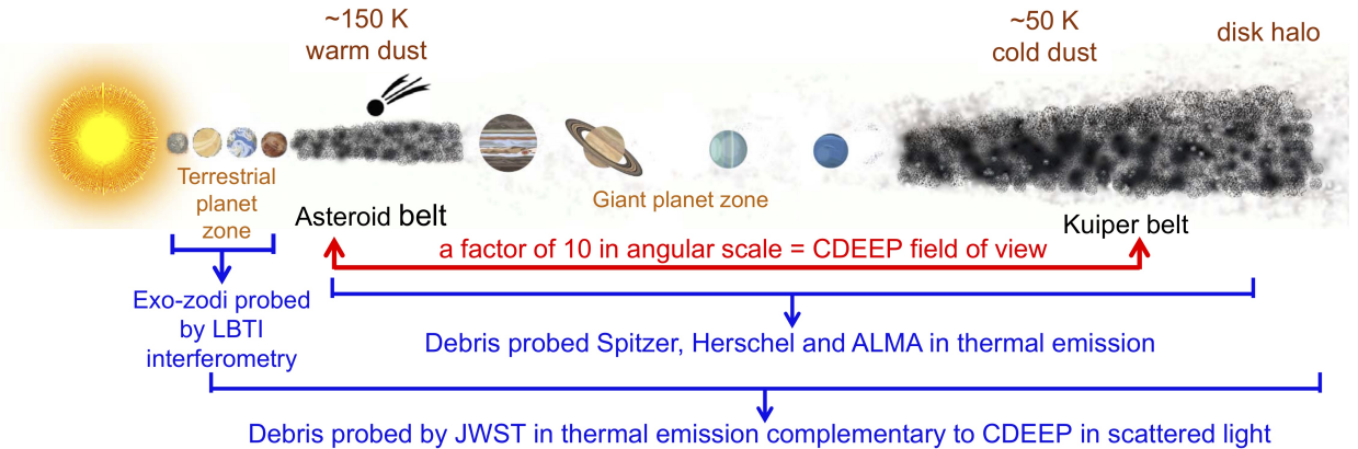
Figure 1: Illustration of the architecture of the solar system where the warm, asteroid-like and the cold, Kuiper-belt-like planetesimal belts are separated by the four giant planets. CDEEP's large field-of-view (FOV), ranging a factor of 10 in angular scale, enables a direct connection between the warm and cold debris in exoplanetary systems. This unique capability probes the debris studied by mostly unresolved IR observations, complementary to the recently completed NASA/Large Binocular Telescope Interferometer (LBTI) exozodi survey 13 and future James Webb Space Telescope (JWST) observations.
