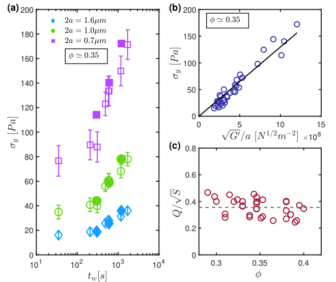
FIG. 3. (a) Macroscopic yield stress (filled symbols) of \phi \simeq 0.35 suspensions as measured from rheology stress sweep tests. Open symbols (in corresponding colors) are the predictions obtained from Eq. (8) using the single value Q \simeq 0.9 for all three series of points. (b) Test of the macroscopic constitutive relation [Eq. (9)]: \sigma_y vs \sqrt{G'}/a for all \phi \simeq 0.35 suspensions, with 2a ranging from 0.7 to 1.6 \mu\text{m} and I from 0.1 to 0.2 M. The solid line is not a fit, but the prediction of Eq. (9) using the \phi -average value of Q/\sqrt{S} \sim 0.355 from panel (c) and the fitted value of g(a^*)/\sqrt{a^*} . (c) Q/\sqrt{S} as a function of \phi , obtained from independent fits of Q and S by matching microscopic and macroscopic data.
