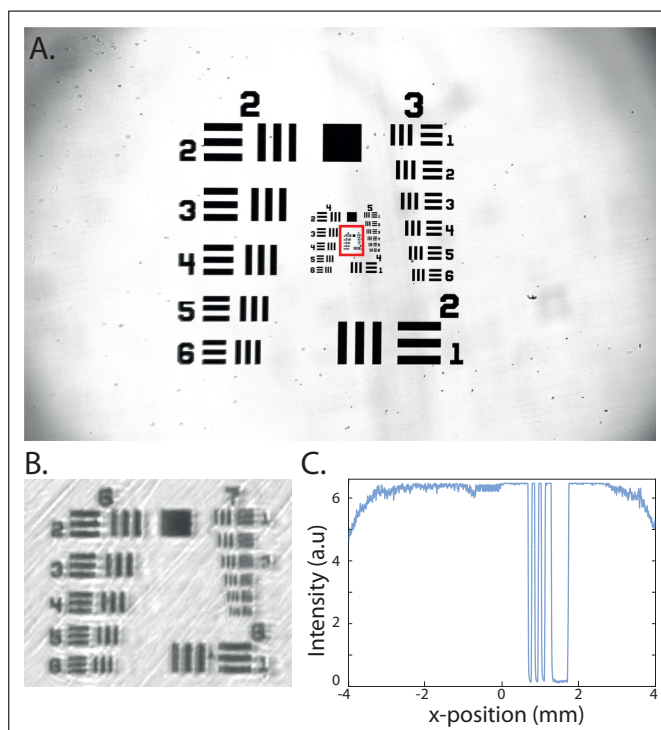
Fig. 2. Optical performances of the Incubascope. (a) Bright-field image of a USAF resolution target. (b) Zoom in of the area highlighted by the red square in (a). The smallest resolvable line is the element 3 of the group 7. (c) Plot of the intensity profile along a line of the image displayed in (a). A decrease of 17 % is observed across the 8 mm FOV.
